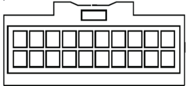
Black 20 Pin Amplifier Bypass Harness (Factory Amp Location)
