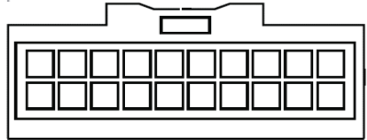
Black 20 Pin Amplifier Bypass Harness (Factory Amp Location)
