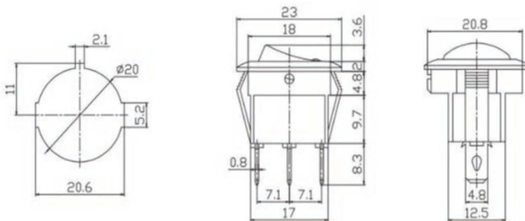
Dimensions (mm)
